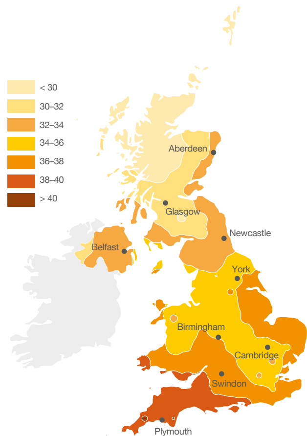
Figure 2. Average annual solar radiation 1981–2010 (TJ/ha)
