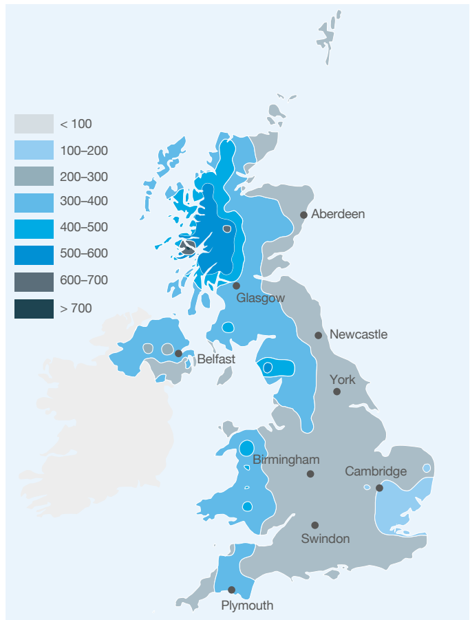
Figure 3. Average rainfall April–July, 1981–2010 (mm)
