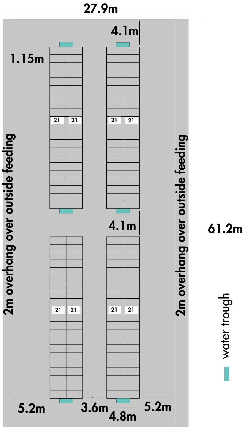
61.2m long (10 x 6.096m bays)
