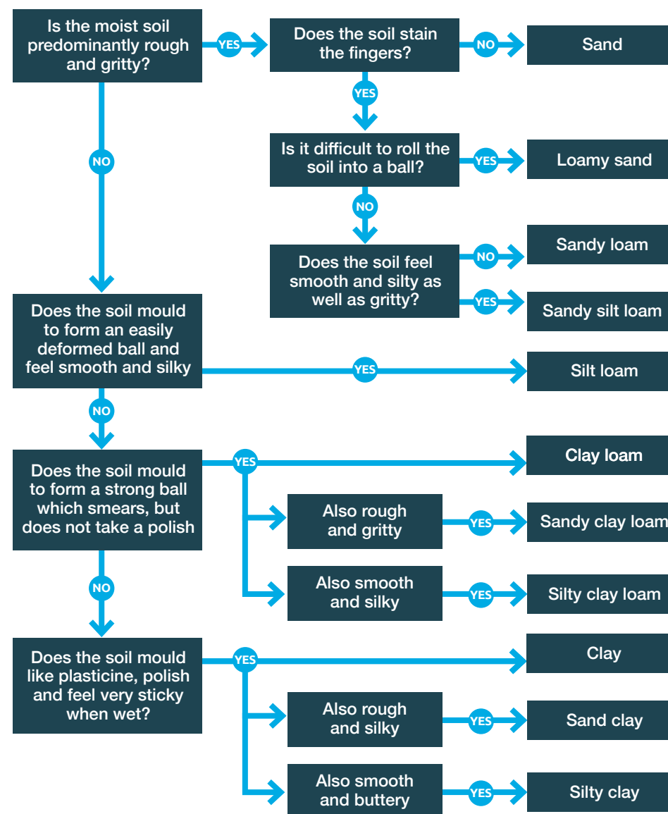
Figure 1.1 Assessment of soil texture by hand
