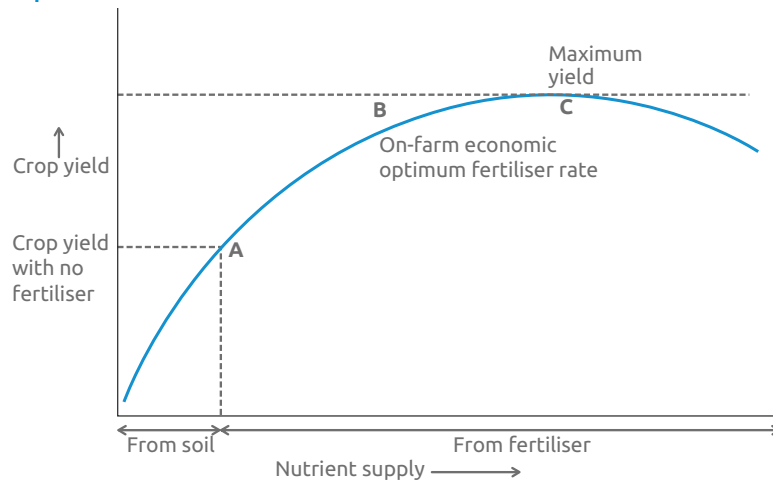
Figure 1.2 A typical nitrogen response curve
