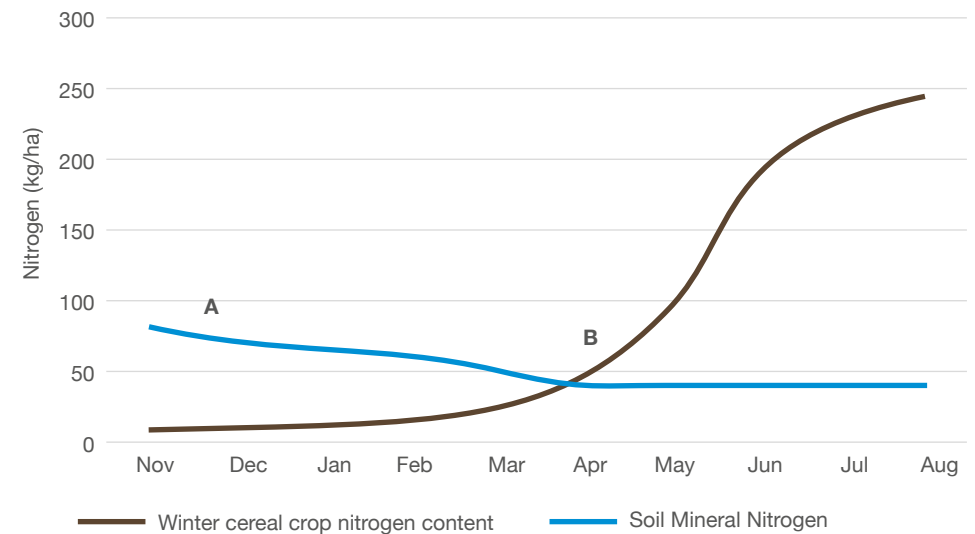
Figure 1.3 Nitrogen uptake by a winter cereal crop in relation to available soil nitrogen
