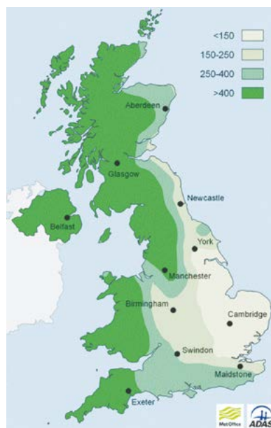
Figure 3.3 Excess winter rainfall (mm)
