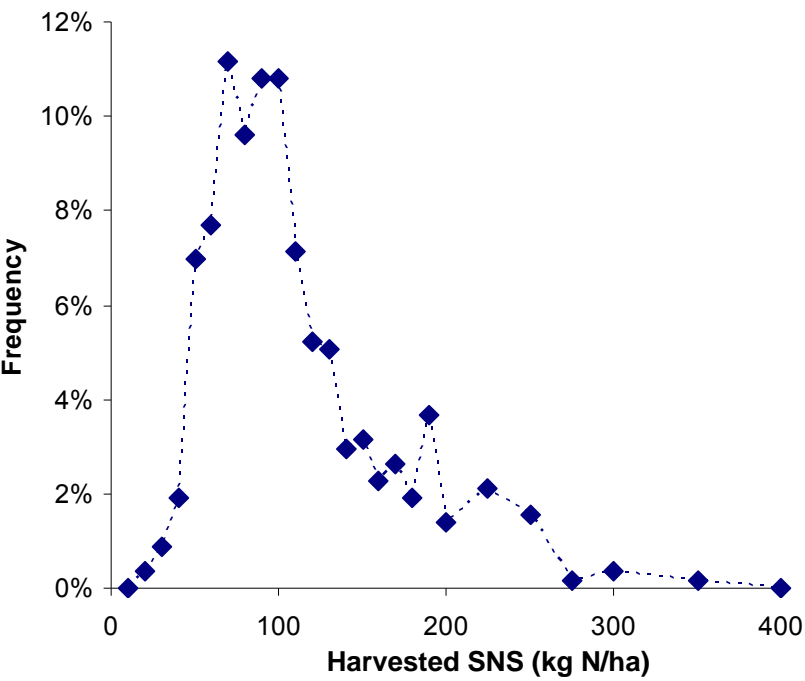
Figure 2. Frequency distribution of harvested SNS for >550 experimental sites in UK since 1980
