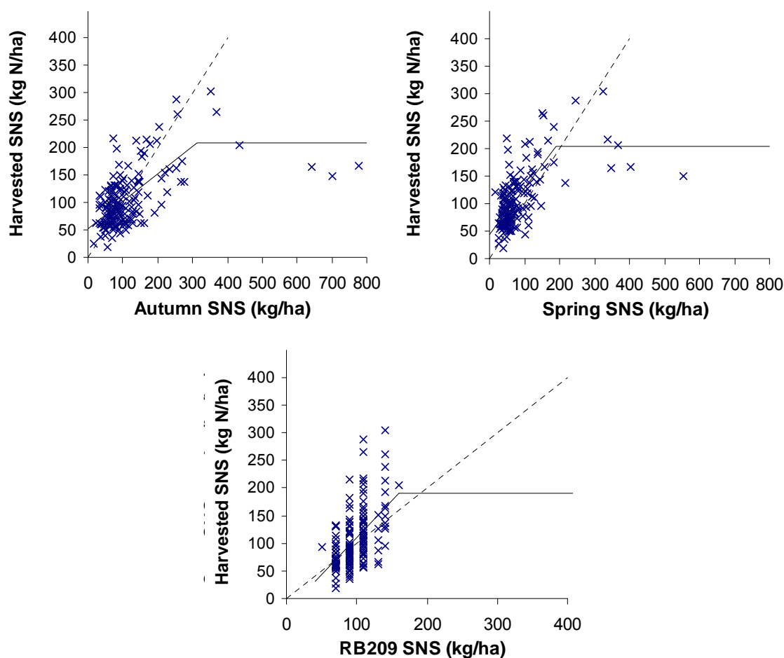
Figure 42. Relationships (with fitted broken stick functions; line) between SNS measured in Autumn (A), Spring (B) or (C) estimated by FAM (RB209) and harvested SNS for 164 sites in 2008-2010. Dotted line: y=x .
