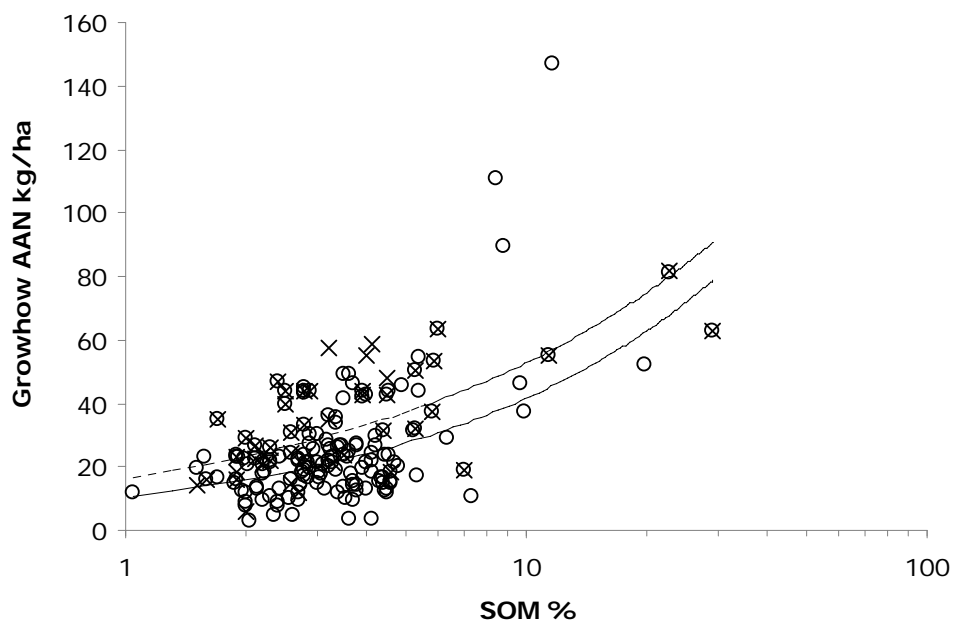
Fig A4.2. Relationship between SOM and Growhow AAN for this current HGCA SNS project data (circles; dashed line) and GrowHow data (crosses; dotted line).
