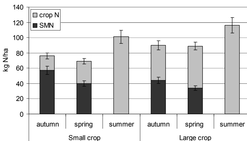
Figure 54. Overall mean SMN (kg/ha) and crop N (kg/ha) in autumn, spring and summer from 2007/08, 2008/09 and 2009/10 with small and large crop treatments. N=28 \pm \text{SEM} per treatment.
