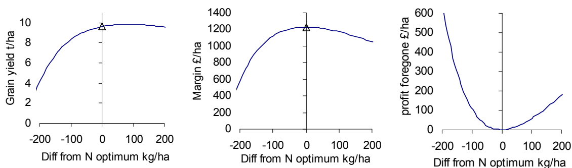
Figure 56. Response curves for grain yield, margin over fertiliser cost (ignoring other costs), thus profit foregone from non-optimal fertiliser use, as used to calculate costs of different approaches to SNS prediction.
