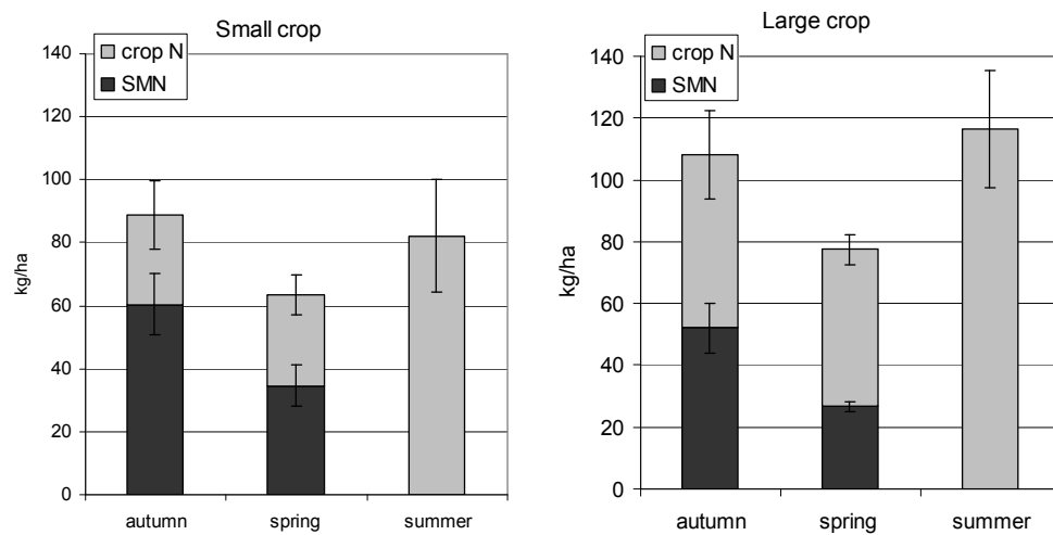
Figure A5.3. Mean SMN (kg/ha) and crop N (kg/ha) in autumn, spring and summer 2009/10 with small and large crop treatments. N=10 \pm SEM per treatment.
