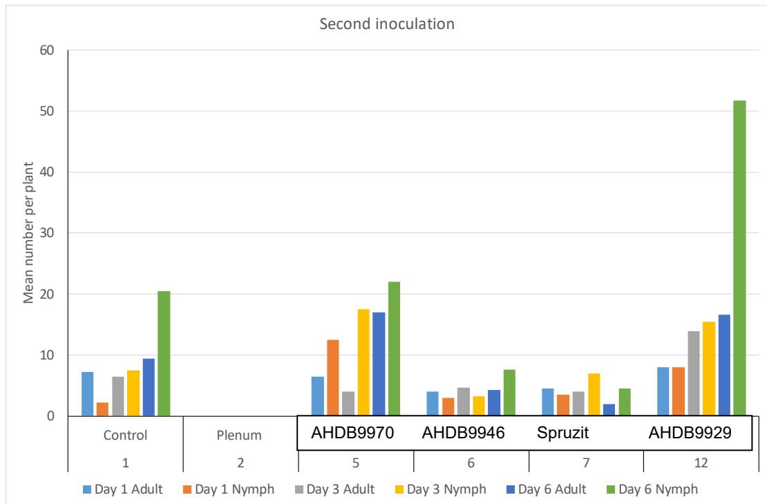
Figure 2b Myzus persicae – survival during the first week after inoculation/treatment with bio-insecticide products, shown as mean number of aphids per plant. Bio-insecticides applied on Day 0 and Day 7.
