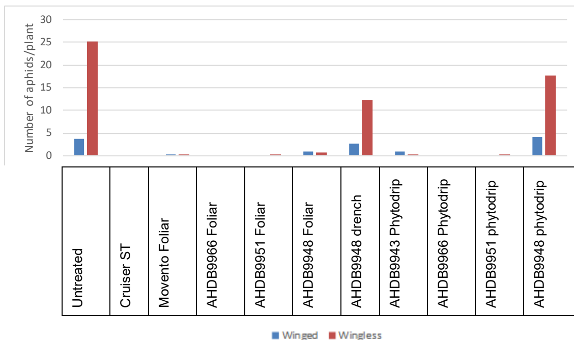
Figure 6 Nasonovia ribisnigri – mean number of winged and wingless aphids per plant on lettuce plants treated 1) at sowing with seed or phytodrip treatments, with foliar sprays or with a pre-planting drench treatment (2 replicates only).
