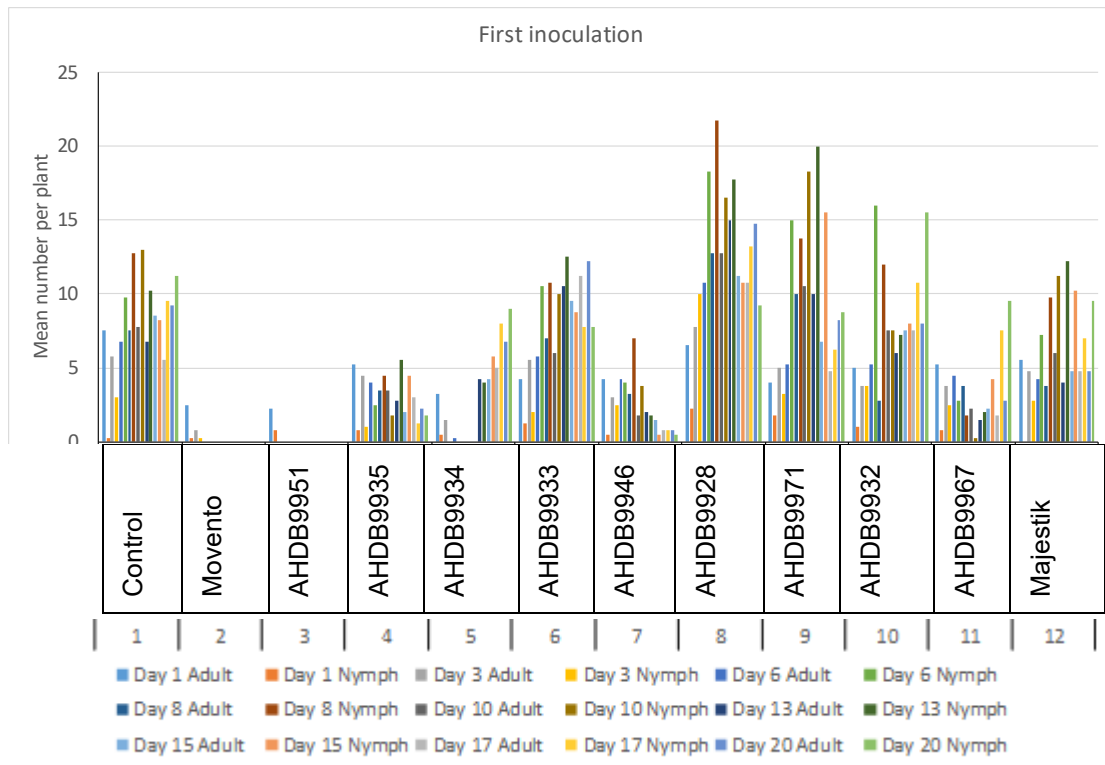
Figure 5a Nasonovia ribisnigri – survival after inoculation/treatment with insecticide and bio-insecticide products shown as mean number of aphids per plant. Insecticides applied on Day 0 and bio-insecticides applied on Day 0 and Day 7.
