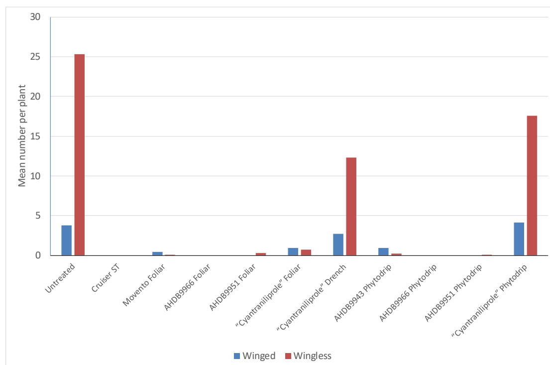
Figure A Nasonovia ribisnigri – mean number of winged and wingless aphids per plant on lettuce plants treated 1) at sowing with seed or phytodrip treatments, with foliar sprays or with a pre-planting drench treatment (2 replicates only).
