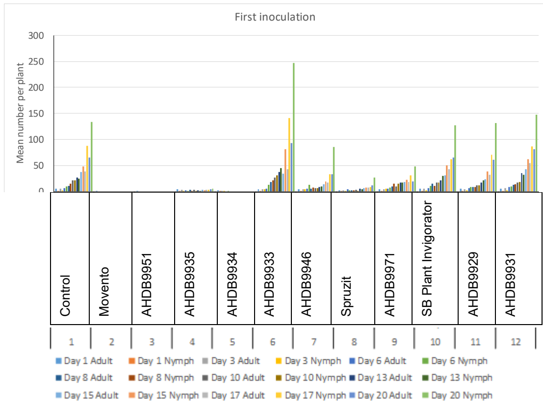
Figure 4a Cavariella aegopodii – survival after inoculation/treatment with insecticide and bio-insecticide products shown as mean number of aphids per plant. Insecticides applied on Day 0 and bio-insecticides applied on Day 0 and Day 7.
