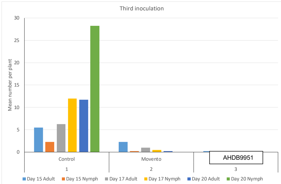
Figure 4c Cavariella aegopodii – survival after inoculation/treatment with insecticide and bio-insecticide products shown as mean number of aphids per plant. Insecticides applied on Day 0 and bio-insecticides applied on Day 0 and Day 7.
