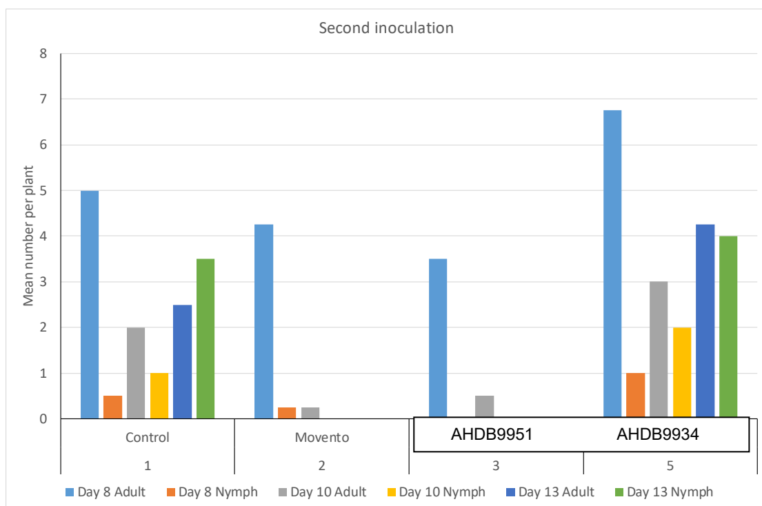
Figure 5b Nasonovia ribisnigri – survival after inoculation/treatment with insecticide and bio-insecticide products shown as mean number of aphids per plant. Insecticides applied on Day 0 and bio-insecticides applied on Day 0 and Day 7.
