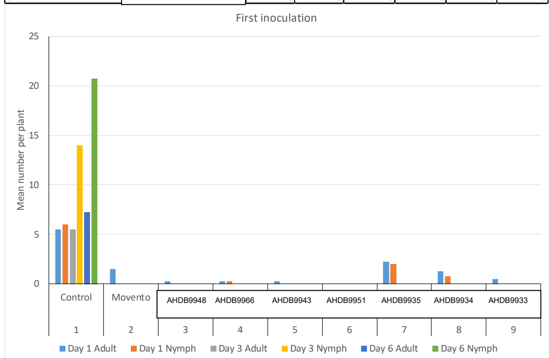
Figure 1a Myzus persicae – survival during the first week after inoculation/treatment with conventional insecticide products shown as mean number of aphids per plant. Insecticides applied on Day 0 and bio-insecticides applied on Day 0 and Day 7.
