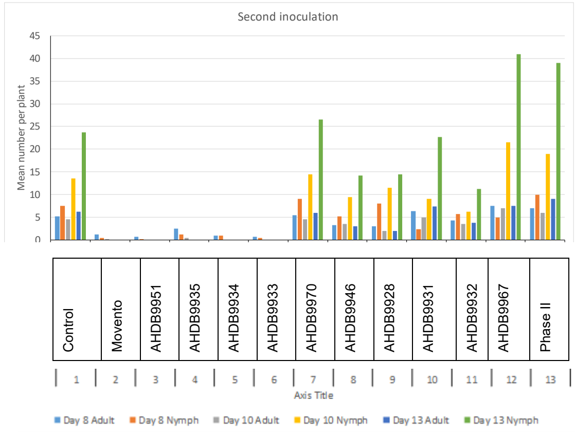
Figure 3a Brevicoryne brassicae – survival after inoculation/treatment with insecticide and bio-insecticide products shown as mean number of aphids per plant. Insecticides applied on Day 0 and bio-insecticides applied on Day 0 and Day 7.
