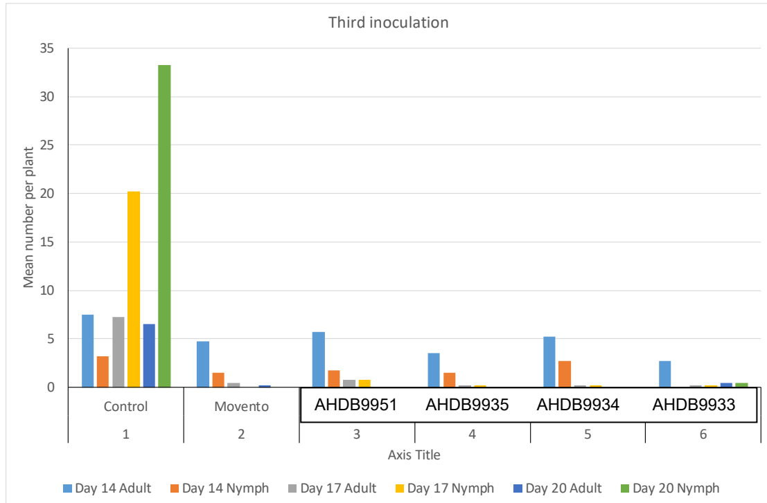
Figure 3c Brevicoryne brassicae – survival after inoculation/treatment with insecticide and bio-insecticide products shown as mean number of aphids per plant. Insecticides applied on Day 0 and bio-insecticides applied on Day 0 and Day 7.
