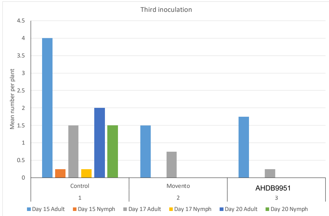
Figure 5c Nasonovia ribisnigri – survival after inoculation/treatment with insecticide and bio-insecticide products shown as mean number of aphids per plant. Insecticides applied on Day 0 and bio-insecticides applied on Day 0 and Day 7.
